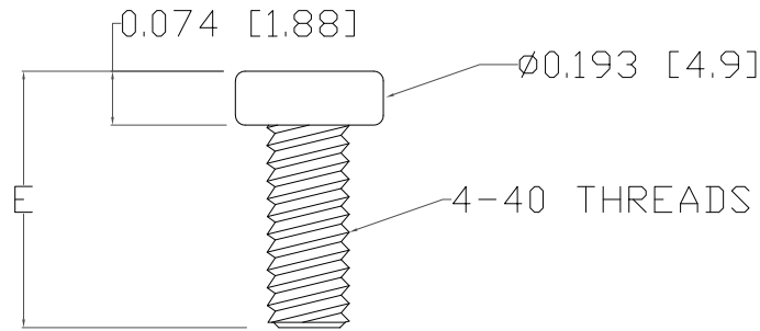
STRAIN RELIEF SCREWS 2-TOTAL
